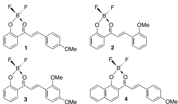
Scheme 1. Molecular structures of compounds 1–4.
