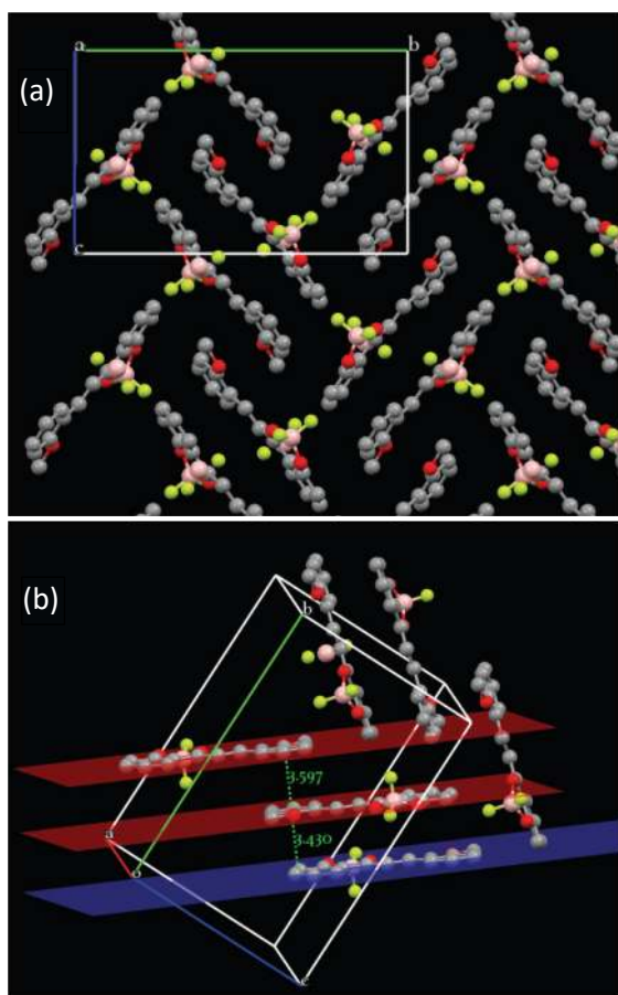
Figure 3. Views of of the crystal structure of dye 3 (a) along a axis and (b) showing details of the two types of pairwise association. Hydrogen atoms were omitted for clarity.
