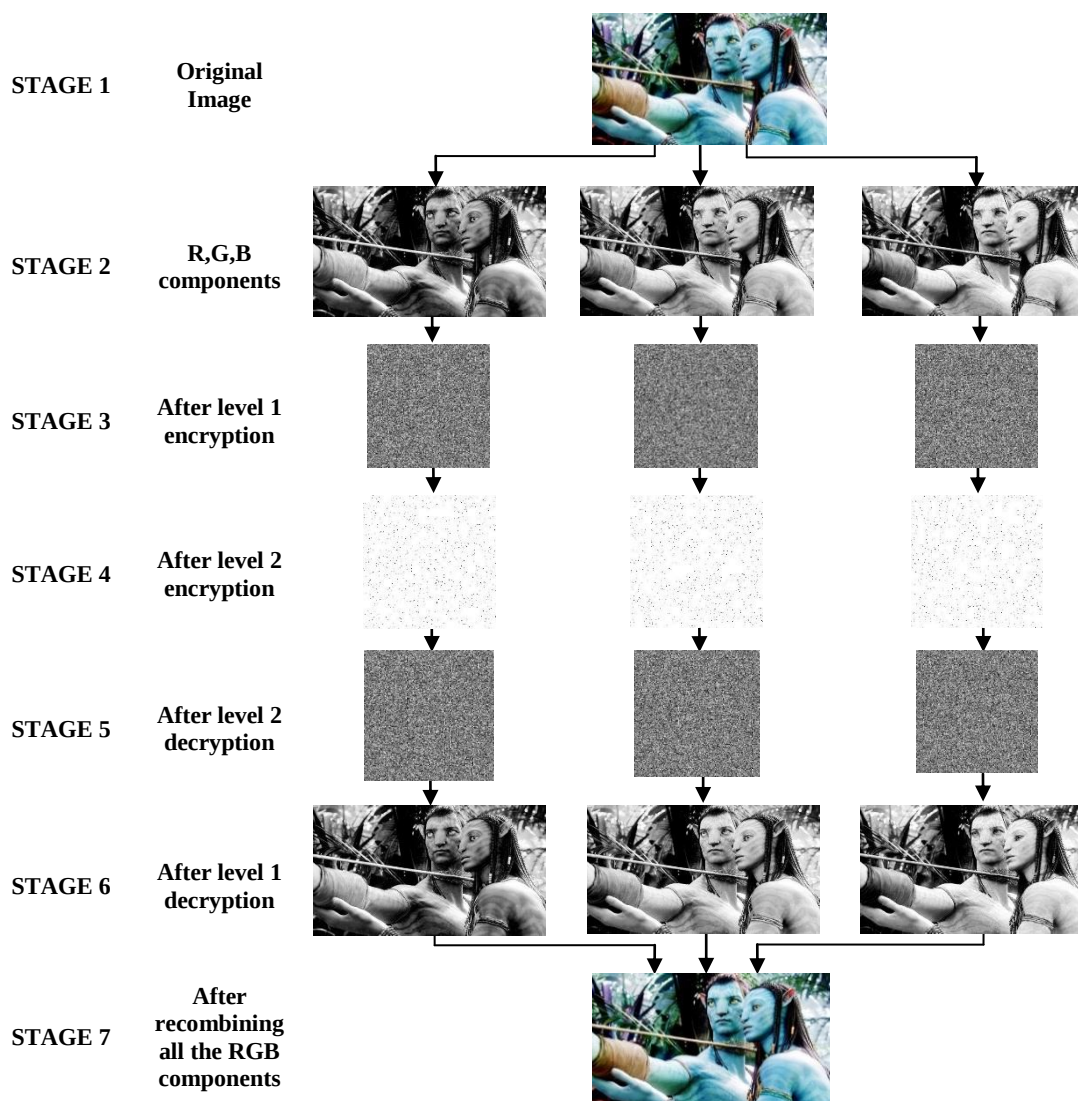
Fig 6: Encrypting and decrypting over the RGB Components
