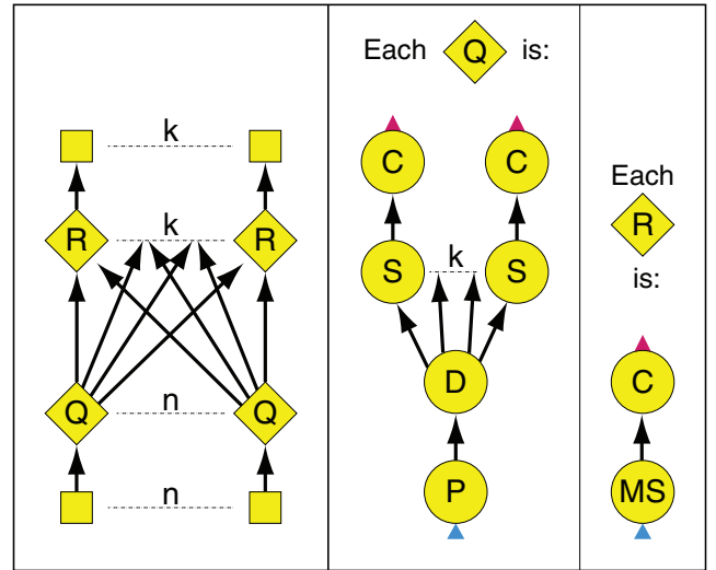
Figure 9: The communication graph to compute a query histogram. Details are in Section 6.3. This figure shows the first cut “naive” encapsulated version that doesn’t scale well.
