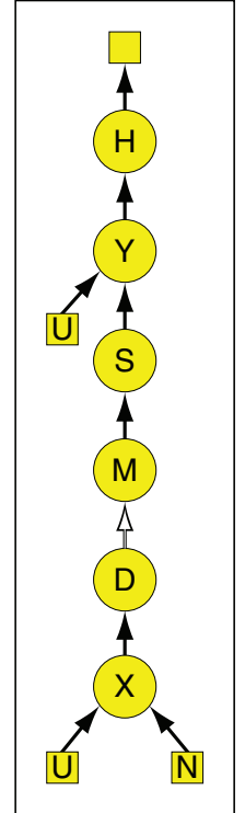
Figure 5: The stages of the Dryad computation from Figure 2. Section 3.6 has details.
