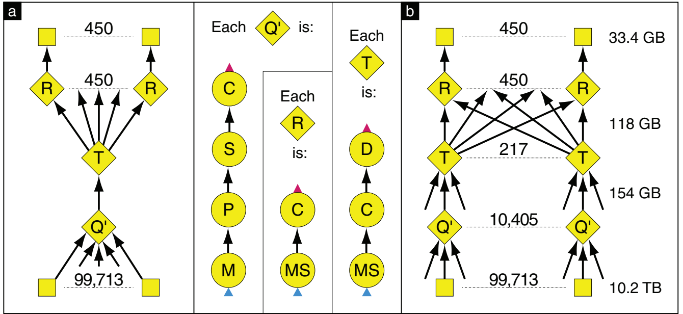
Figure 10: Rearranging the vertices gives better scaling performance compared with Figure 9. The user supplies graph (a) specifying that 450 buckets should be used when distributing the output, and that each Q' vertex may receive up to 1GB of input while each T may receive up to 600MB. The number of Q' and T vertices is determined at run time based on the number of partitions in the input and the network locations and output sizes of preceding vertices in the graph, and the refined graph (b) is executed by the system. Details are in Section 6.3.
