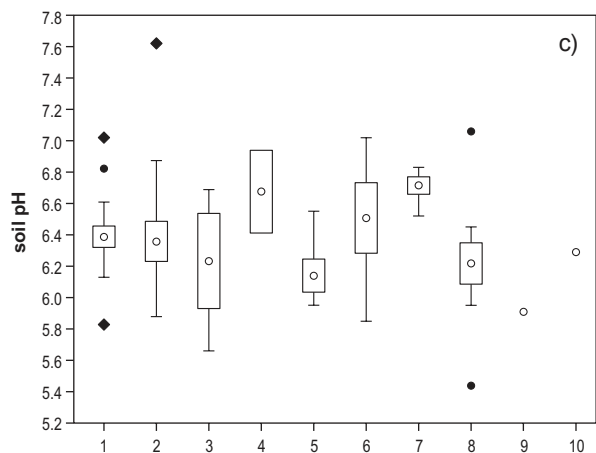
Figure 3: Diagrams for a) humus content, b) total N content and c) pH of soils for the ten studied plant communities.
