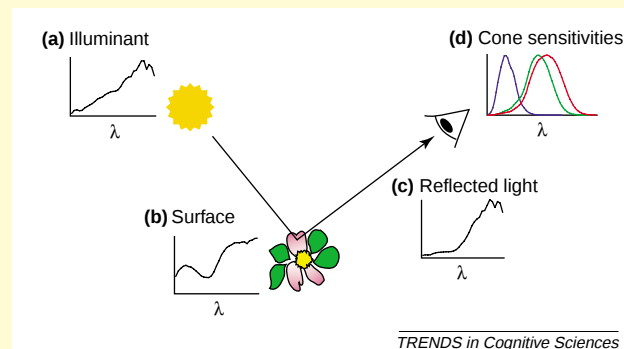
Fig. 1. Sampling spectra. Light from an illuminant with spectrum (a) is reflected by a surface with spectral reflectance (b) ( \lambda = wavelength). The reflected light with new spectrum (c) is absorbed by the eye's cone receptors with spectral sensitivities (d). From this activity in the cones, the visual system has to estimate the surface reflectance (b). Note the change in spectral shape from (b) to (c).
