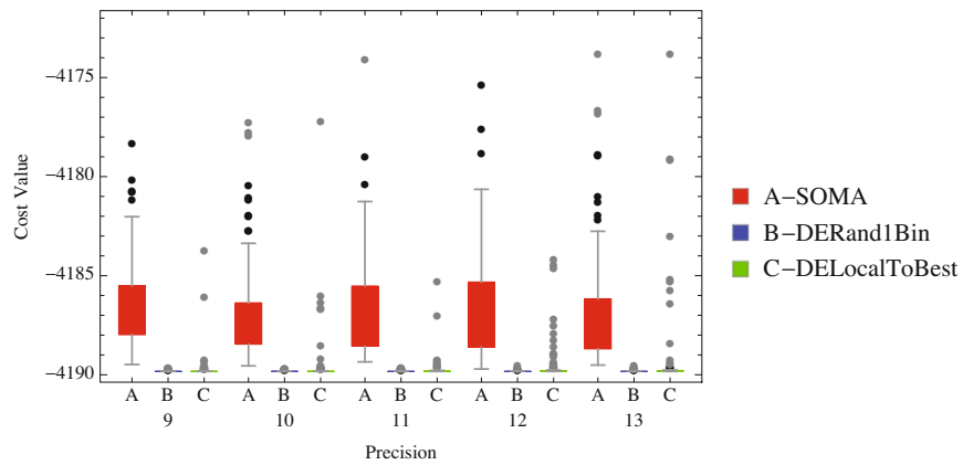
Fig. 4 Case 1. Dependence of algorithm performance on precision - detail with outliers.
