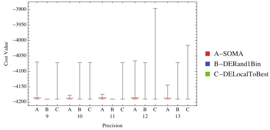
Fig. 3 Case 1. Dependence of algorithm performance on precision - detail.
