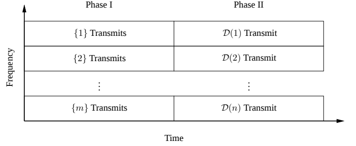
Fig. 2. Example channel allocations across frequency and time. \mathcal{M} = \{1, 2, \dots, m\} denotes the set of cooperating terminals in the network. For source s , \mathcal{D}(s) denotes the set of decoding relays participating in a space-time code during the second phase.
