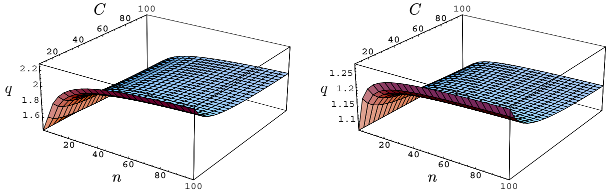
Figure 2: Illustration of the behavior of q under power-law demand for two values of the skewness parameter: a = 0.4 (left graph) and a = 0.8 (right graph). The access costs are: t_l = 0, t_r = 1, t_s = 2 .
