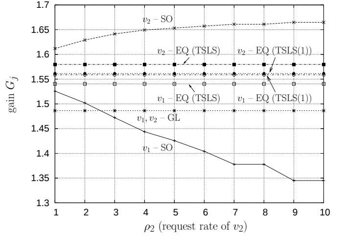
Figure 3: Individual node gains for the example of Table 5. “ v_j - XX ” denotes the gain for node v_j under the placement strategy XX .
