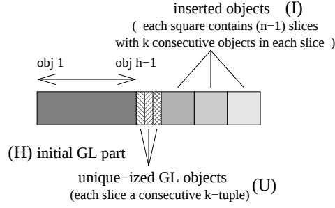
Figure 4: Tomography of the objects that are replicated at a node after the end of TSLS( k ). (H) denotes the set of objects that belong to the “head” of the GL placement, i.e., objects that are left intact by the improvement step because they are too valuable. (U) denotes the set of unique-sized objects, that is objects that were on the GL placement of all the nodes but were subsequently eliminated from all the nodes but the local one. (I) denotes the set of objects that were inserted locally by the improvement step.
