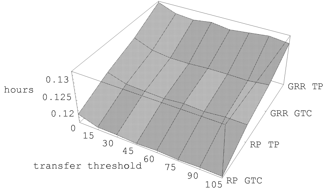
Figure 10. Effect of transfer threshold for N = 32 on 30,915 designs.
