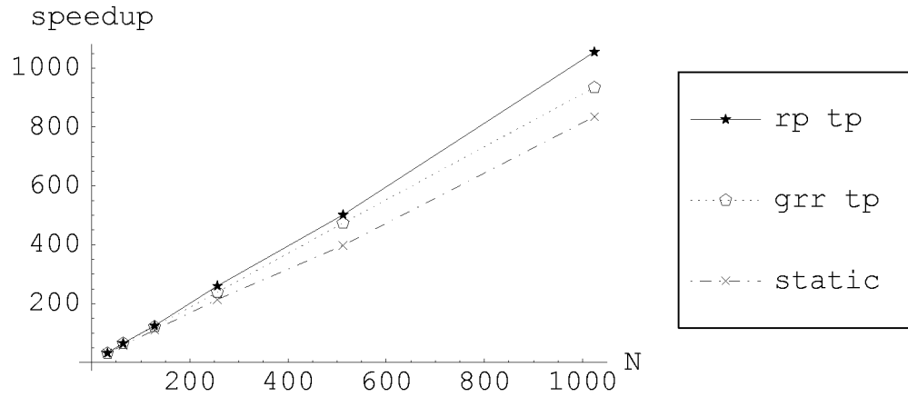
Figure 9. Speedup with base N = 32 for RP and GRR-MC with token passing, on N = 2^{\{5 \dots 10\}} processors.
