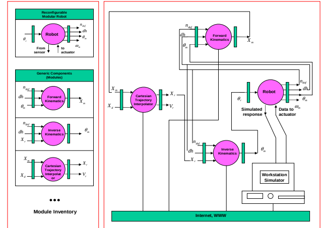
Fig.12: Shared design workspace
