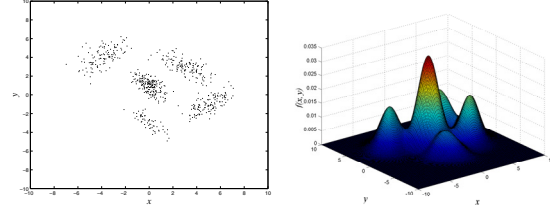
(a) The 2D dataset.
