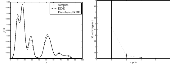
(a) The 1D dataset and estimation results.
