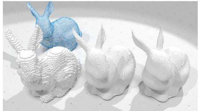
Fig. 13. Voxel upscaling: starting from a low resolution Bunny object ( 64^3 ), we can reconstruct its surface (blue piecewise smooth surface) and use it to upscale the input object to 256^3 and 512^3 resolutions (middle and right).
