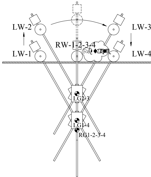
Figure 8 Obstacle-navigation process (first single support phase)
