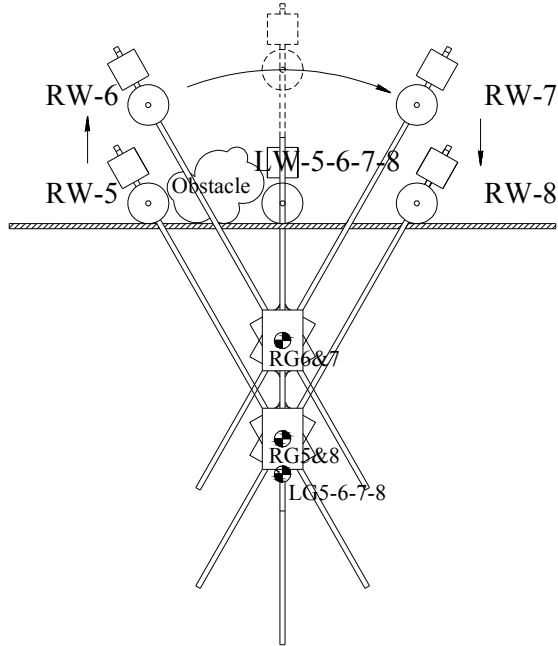
Figure 10 Obstacle-navigation process (final single support phase)
