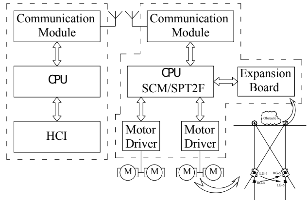
Figure 11 Architecture of the control system
