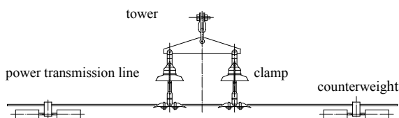
Figure 1 Obstacles on power transmission line
