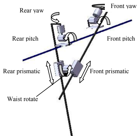
Figure 2 Structure of line-walking robot
