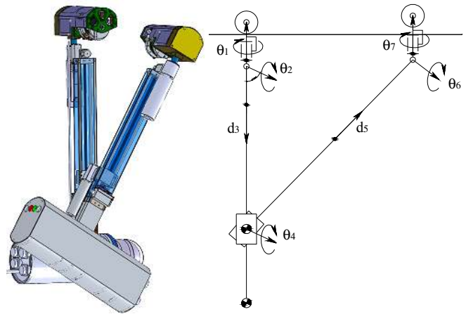
Figure 3 Structure of power transmission line inspection robot
