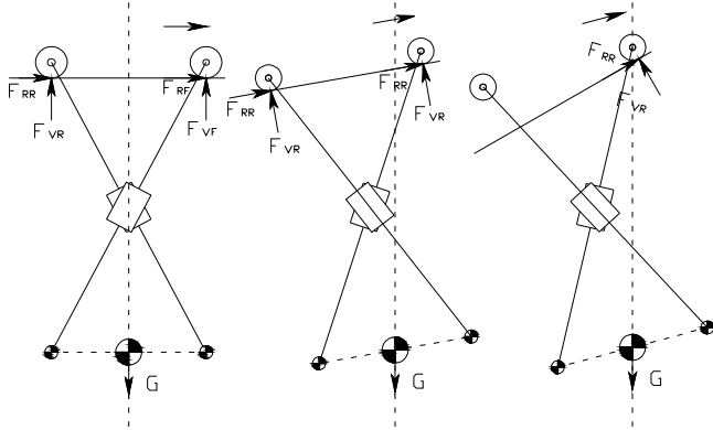
(1) horizontal line (2) less inclination line (3) large inclination line Figure 5 Forces and states analysis with different inclination angle
