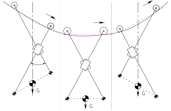
Figure 7 Power transmission line inspection robot based on novel line walking mechanism
