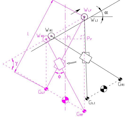
Figure 6 Pose adjustment process
