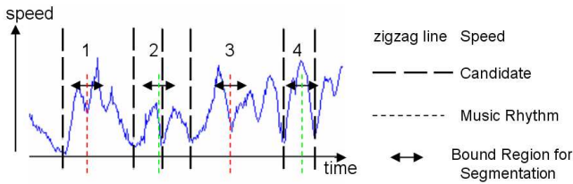
Figure 7: Refinement of the segmentation with musical rhythm
