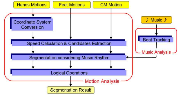
Figure 1: Algorithm Overview
