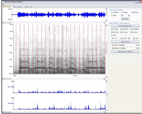
Figure 8: Result - Beat Tracking of Aizu-bandaian
