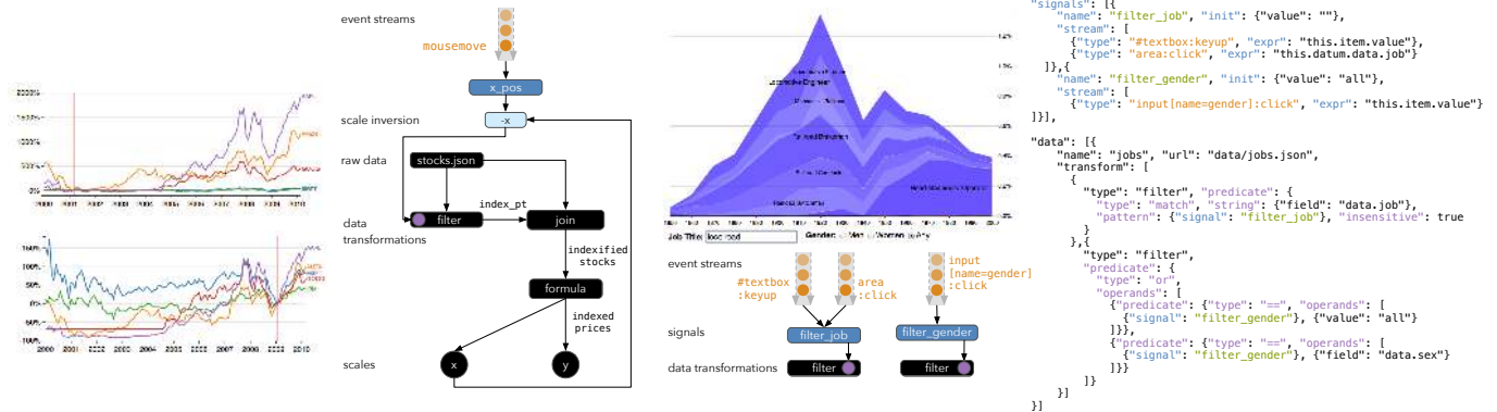
Figure 8. (left) An index chart that shows the percentage changes for a collection of time-series. The index point (red vertical line) is determined by the x position of a mousemove signal. (right) The job voyager can be filtered using signals bound to the state of control widgets. A textbox allows for pattern-based filtering of job titles while radio buttons allow gender-based filtering.
