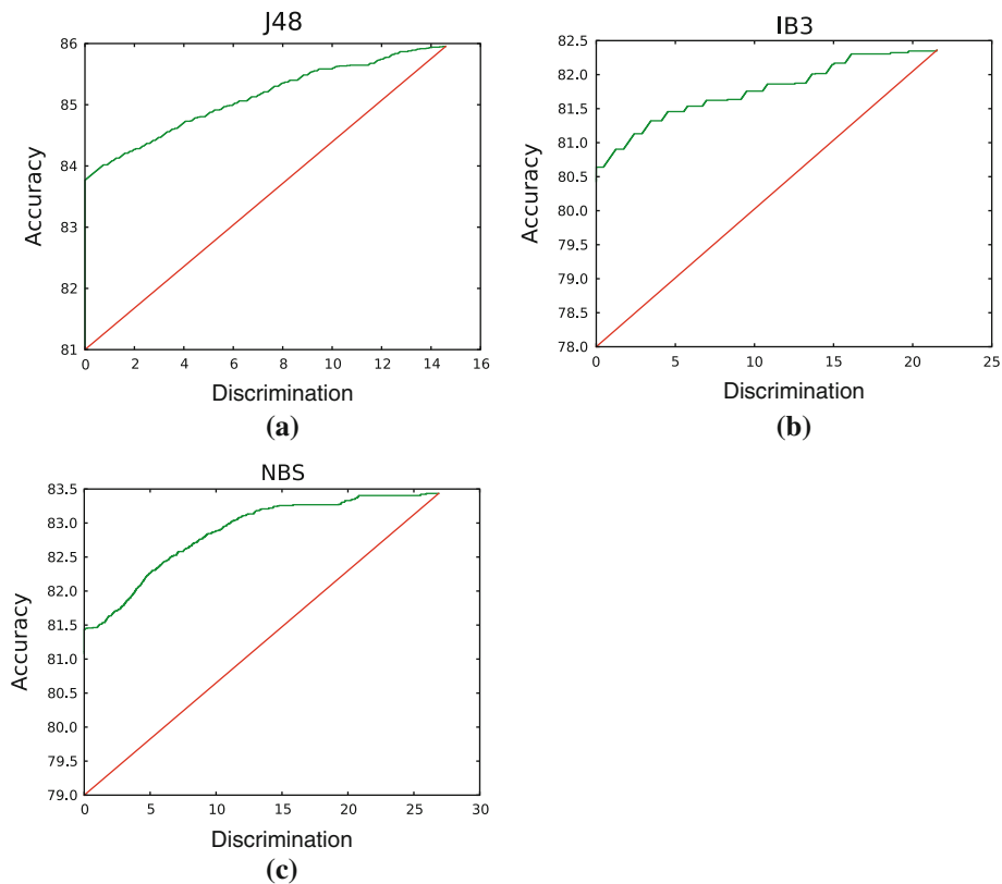
Fig. 1 Trade-off between accuracy and discrimination (dependence) for the DA-optimal classifiers in \mathcal{C}_R and \mathcal{C}_C . a Decision tree. b IBk. c Naïve Bayes
