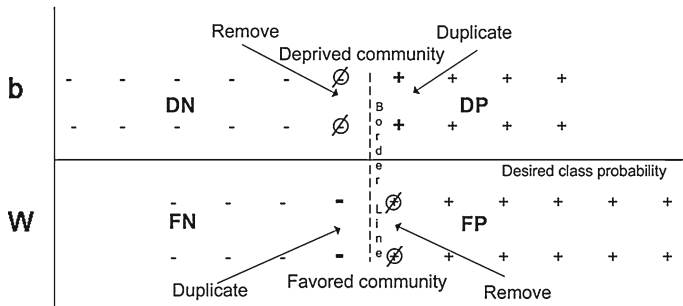
Fig. 4 Pictorial representation of the Preferential Sampling scheme. The re-substituted data points are in bold while the encircled ones are skipped
