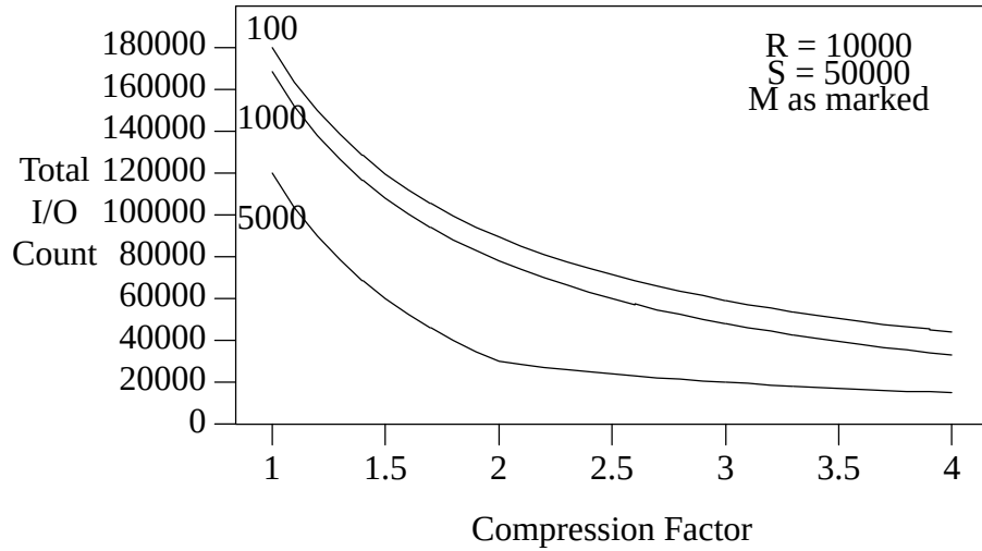
Figure 4. Effect of Compression on Large Hybrid Hash Join Performance.
