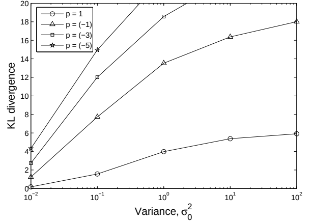
(a) CDKF
