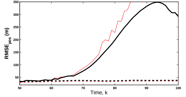
(a) RMSE in position.
