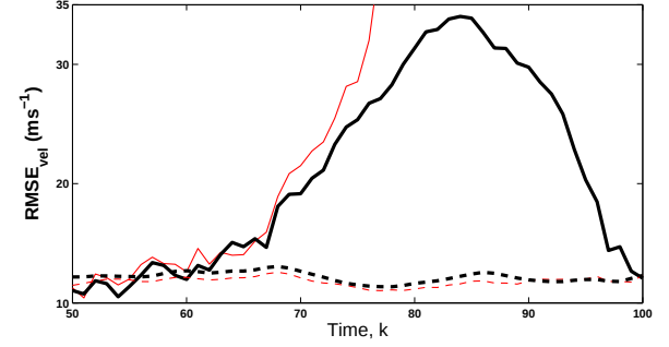
(b) RMSE in velocity.
