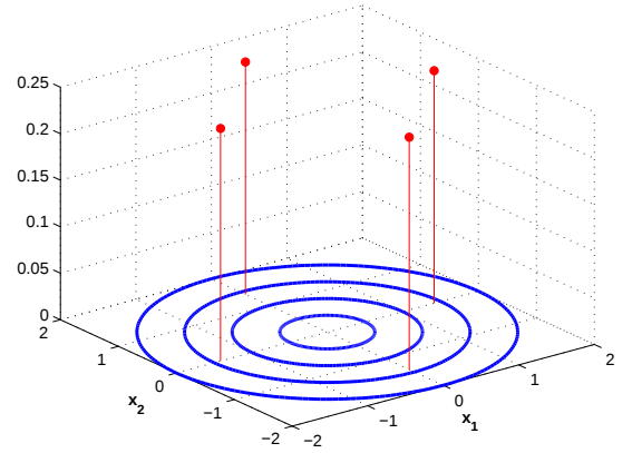
(b) Third-degree spherical-radial cubature point set for the CKF
