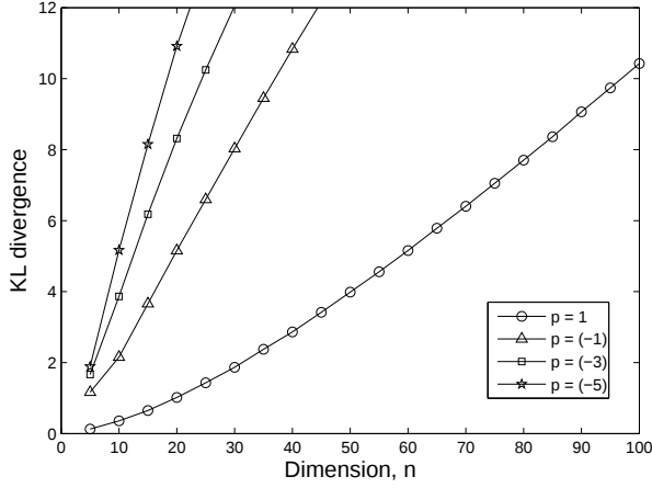
(a) CDKF
