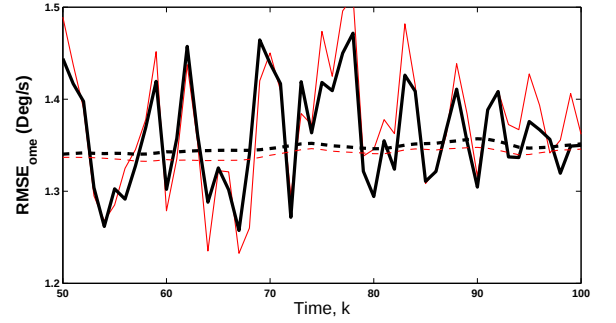
(c) RMSE in turn rate.
