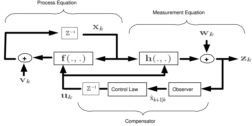
Fig. 1. Signal-flow diagram of a dynamic state-space model driven by the feedback control input. The observer may employ a Bayesian filter. The label \mathbb{Z}^{-1} denotes the unit delay.
