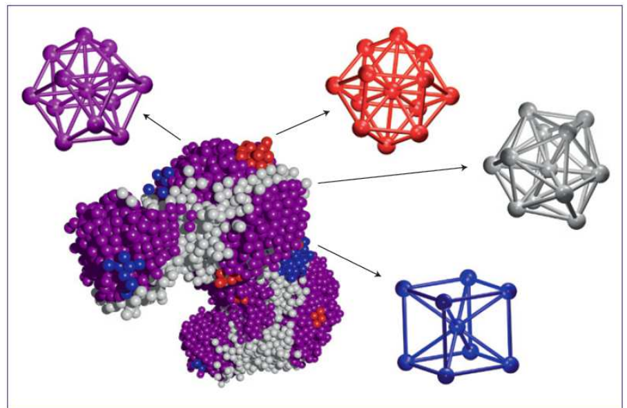
Fig. 1 | Crystal nucleation in colloidal suspensions is a two-step process, the first of which involves the formation of amorphous precursors with different types of short-range order. The existence of domains with hcp-like (purple), fcc-like (red) and bcc-like (blue) order is confirmed by Tan et al. 1 , who have analysed sequences of microscopy images taken from micrometre-sized spherical colloids (represented as coloured balls here) in a solvent. The presence of a domain with liquid-like short-range order (grey) may be expected on the basis of dynamical density functional theory 8 . In the second step, the precursors evolve into nuclei with fcc, bcc or hcp structure. The enlarged purple, red and blue clusters show a central particle surrounded by its nearest neighbours in ideal hcp, fcc and bcc environments, respectively. The crystal-like short-range order can be obtained by distorting these ideal crystalline first-neighbour clusters. To exemplify the liquid-like neighbourhoods, a cluster with neighbouring particles lying on the vertices of a distorted icosahedron is shown.
