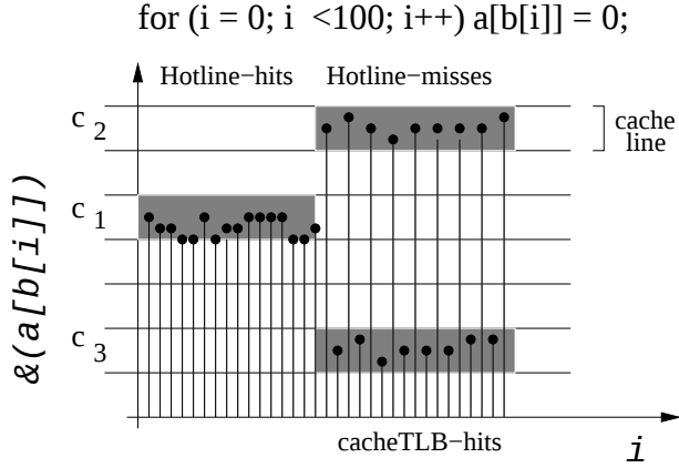
Figure 4: Hotline-misses hitting the Tag-Cache. We found that aggressively speculative hotline accesses that cause hotline-misses, hit the Tag-Cache with good probability.
