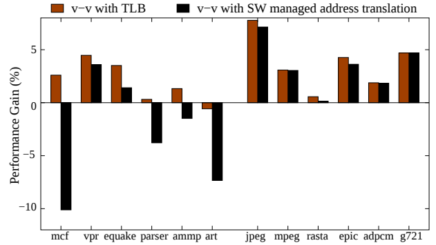
Figure 14: v-v performance: with TLBs vs with software managed address translation
