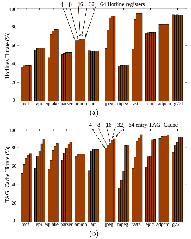
Figure 11: Sensitivity to Hotline register-file and TAG-Cache sizes
