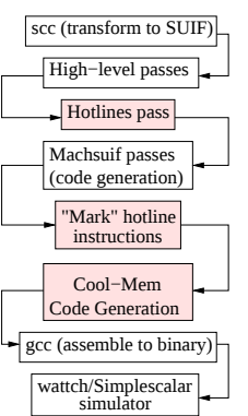
Figure 7: Shaded steps are introduced by Cool-Mem.
