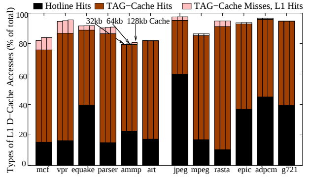
Figure 13: Hitrate sensitivity to Cache size
