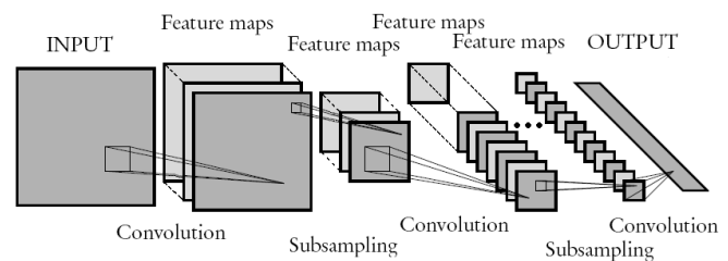
Fig. 1. CNN architecture.
