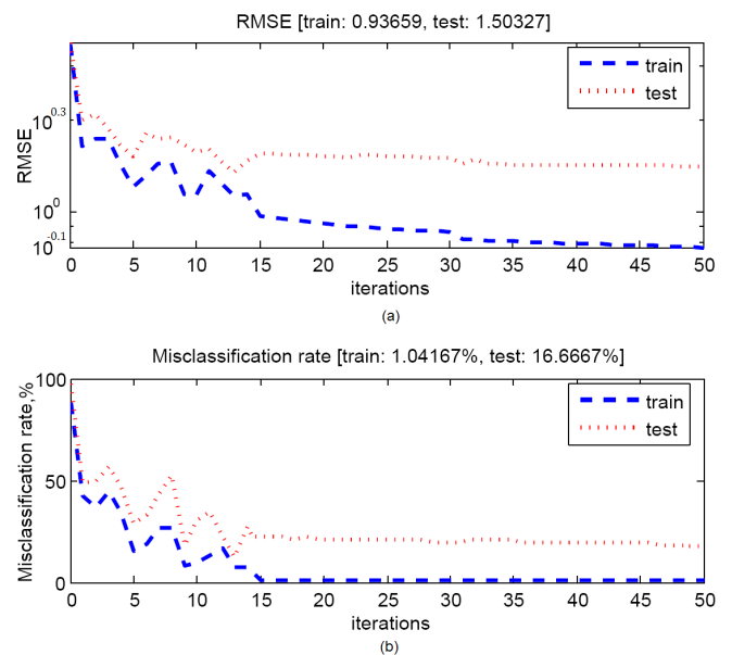
Fig. 5. Performance plot for approximation part of transformed original image: RMSE (a); misclassification rate (b).
