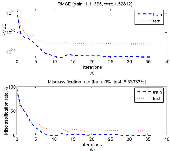
Fig. 6. Performance plot of modified LeNet5: RMSE (a); misclassification rate (b).
