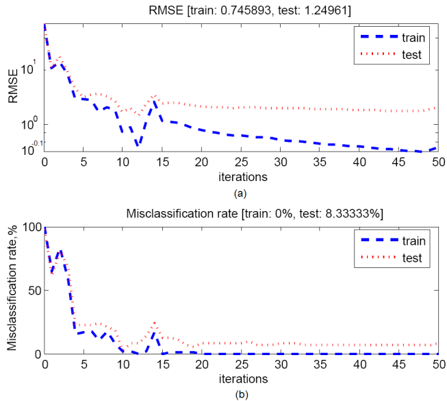
Fig. 3. Performance plots for usual training set: RMSE (a); misclassification rate (b).
