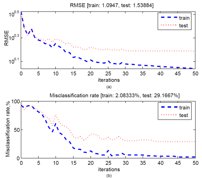
Fig. 4. Performance plot with (5) applied to samples: RMSE (a); misclassification rate (b).
