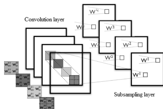
Fig. 2. Subsampling layer formation.
