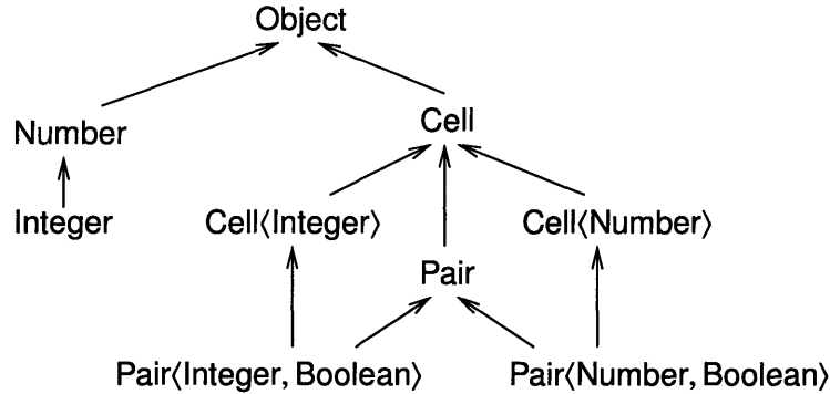
Figure 2-1: A portion of the subtype relation for JSR-14, which uses invariant parametric subtyping. Arrows point from subtypes to supertypes. Classes Cell and Pair are defined in Figure 2-2.
