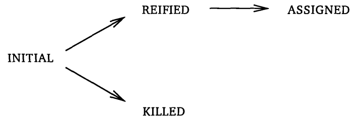
Figure 5-5: States in the declaration type inference algorithm for each type unknown. At each step, every type unknown is associated with a state: initially the INITIAL state, and at completion, either the ASSIGNED or KILLED state. Edges indicate the permitted transitions between states; only during backtracking is a previous state restored.
