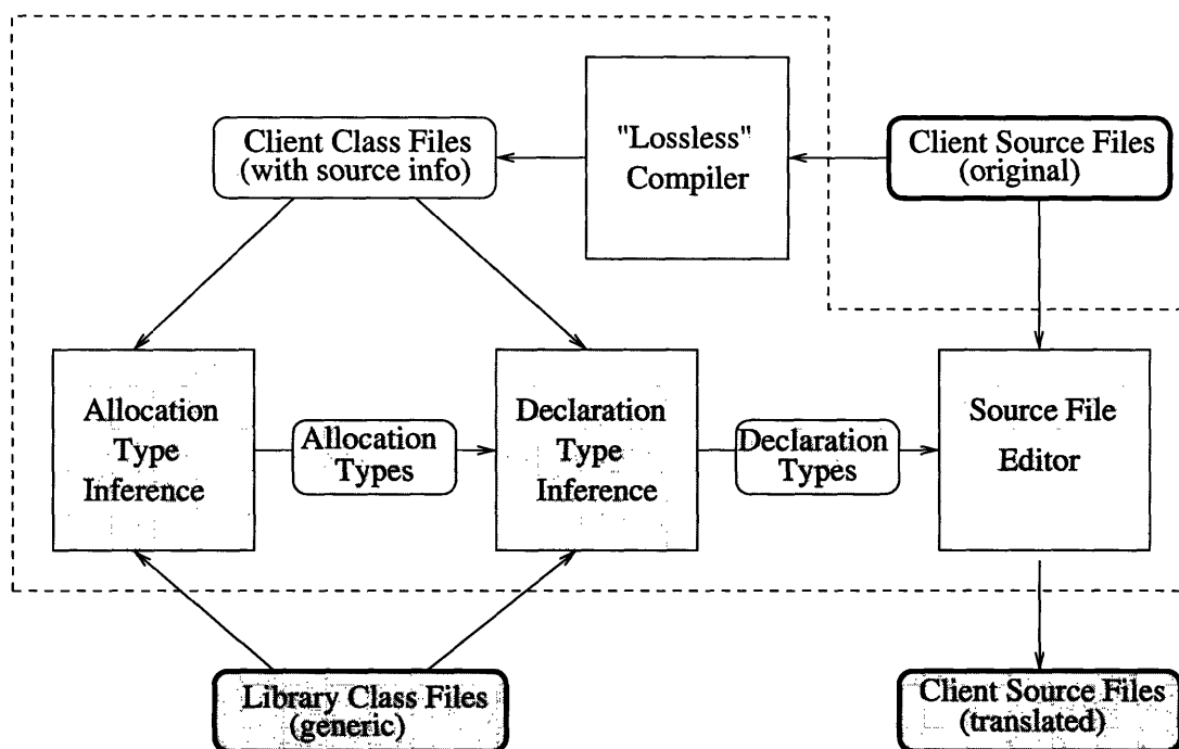
Figure 6-1: Architecture of the Jiggetai tool for automatic translation from Java to JSR-14. Rectangles denote program components; rounded boxes denote data. The dashed border delimits Jiggetai itself; inputs and outputs are shown with heavy outlines.
