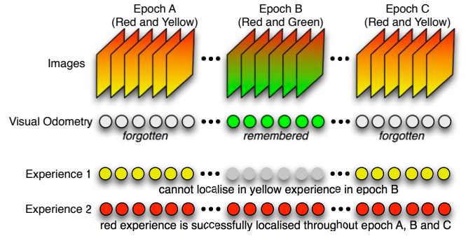
Fig. 1. An outline of our previous work. While traversing an environment a stereo camera produces a stream of frames. A visual odometry (VO) system consumes these to estimate motion and landmark positions. In this example, the decision to save or discard the VO output is a function of the ability to localise against experience 1 and 2. In epochs A and C the live frame stream is successfully localised against both experiences, meaning the VO output is not saved. However in epoch B only experience 2 is localised against the live frame. In this example we require the minimum number of successful localisers to be 2, so in this region a new experience is created from the VO output. This figure is reproduced from [1].
