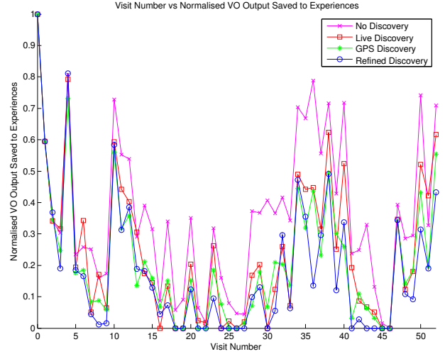
Fig. 5. System performance when using different graph structure discovery approaches. N = 1 for all runs.
