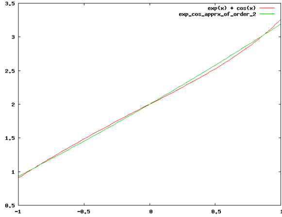
Fig. 4. Approximating \exp(x) + \cos(x) using Chebyshev
