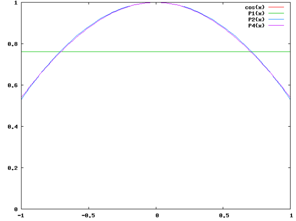
Fig. 1. Approximating \cos(x) using Chebyshev
