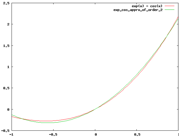
Fig. 5. Approximating \exp(x) - \cos(x) using Chebyshev
