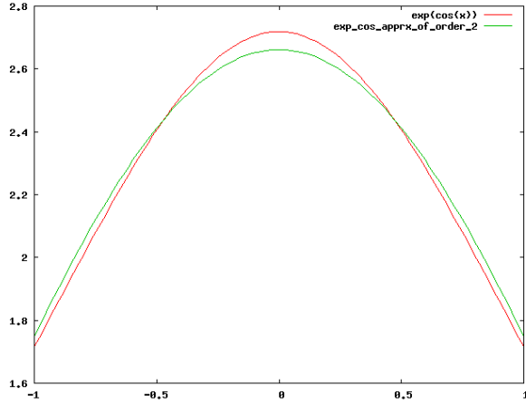
Fig. 7. Approximating \exp(\cos(x)) using Chebyshev
