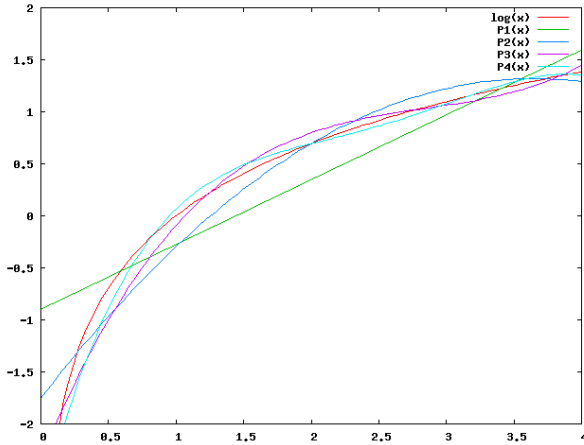
Fig. 3. Approximating log(x) using Chebyshev
