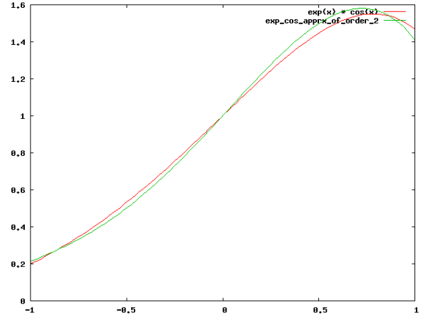
Fig. 6. Approximating \exp(x) * \cos(x) using Chebyshev
