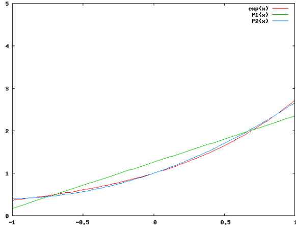
Fig. 2. Approximating exp(x) using Chebyshev
