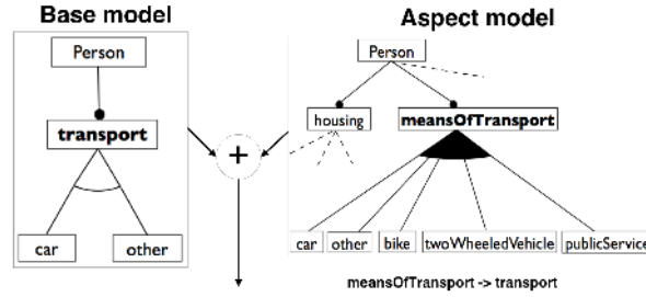
(a) Base and Aspect FMs to be merged
