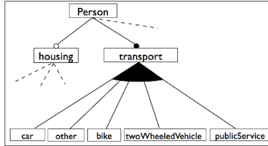
(b) Merged FM
