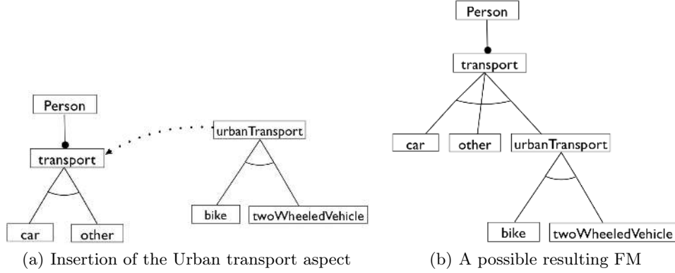
Fig. 3. Example of insertion of FM
