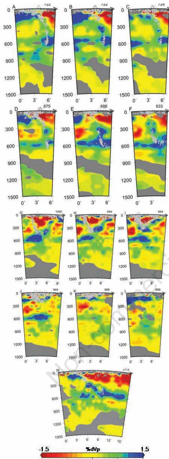
Figure 4. Vertical sections across the convergent margin in the contorted Banda arc through the P-wave model plotted as velocity perturbations relative to ak135 . Vertical sections A-F are around the Timor trough. Vertical sections G-L are across the southern (Aru trough) and northern (Seram trough) arms of the Banda arc; while M trending east-west depicts the deflected slab in the mantle transition zone. Contour scales are from -1.5\% to +1.5\% . Circles depict earthquake hypocenters projected from a distance of up to 55 km on both sides of the plane of section. For each region, the cross section length is listed at the top-right in km, and in degrees at the bottom-right. Grey depicts mantle regions of poor sampling.
