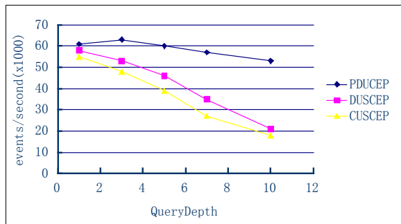
Figure 7. Performance For Different Query Depth
