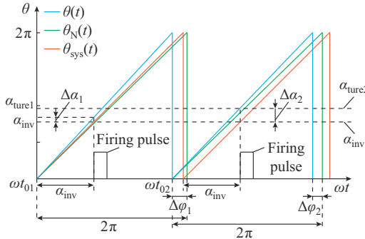
Fig. 2. Relationship between \theta(t) , \theta_{\text{sys}}(t) , and \theta_{\text{N}}(t) .
