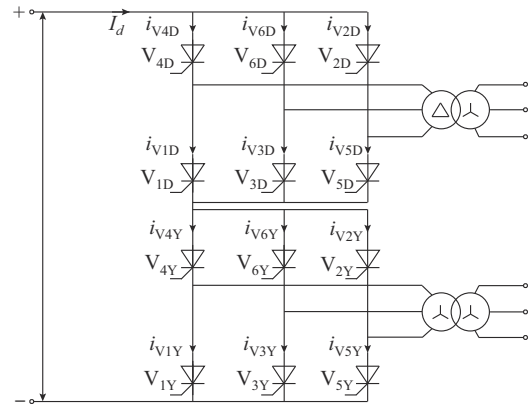
Fig. A1. Twelve-pulse converter at inverter side.
