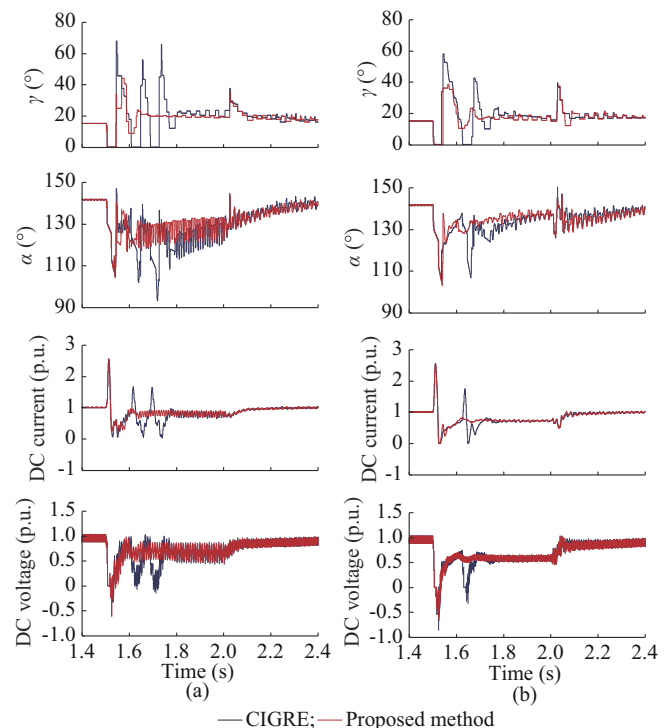
Fig. 8. System response under different faults with different control methods. (a) A-G fault. (b) ABC-G fault.
