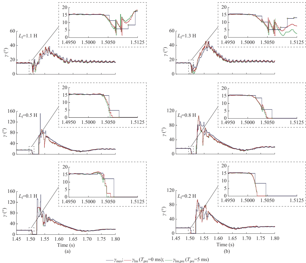
Fig. 5. Waveforms of imaginary EA ( \gamma_{lm}(T_{pre}=0\text{ ms}) and \gamma_{lm,pre}(T_{pre}=5\text{ ms}) ) and measured EA \gamma_{mes} under different faults. (a) A-G faults with different L_f . (b) ABC-G faults with different L_f .
