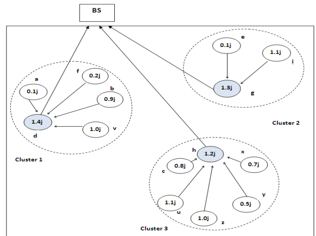
Fig2. Cluster formation of First round
