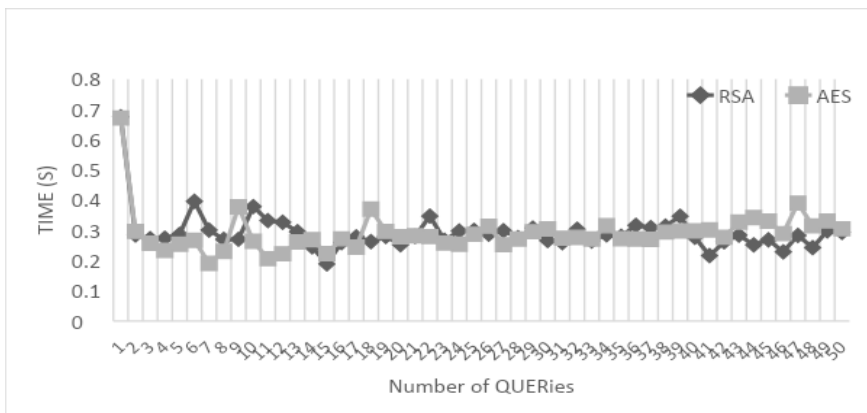
Graphic 7. Decryption Time for Delete.
