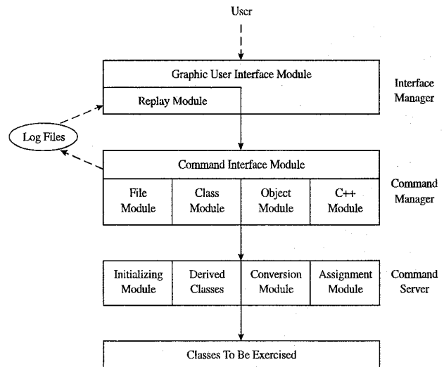
Figure 2: The Structure of RunClass
