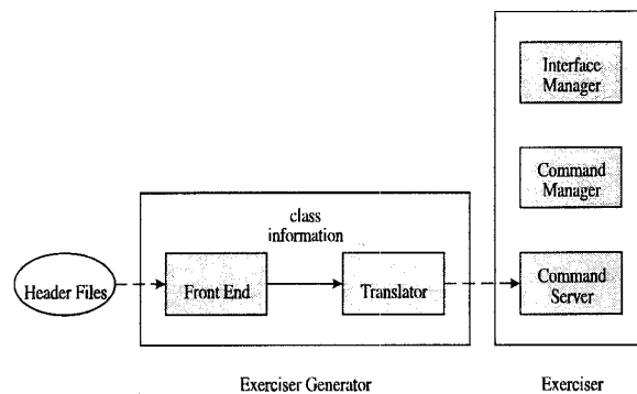
Figure 1 The Components of RunClass
