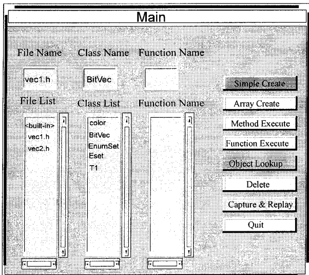
Figure 3. The Main Menu
