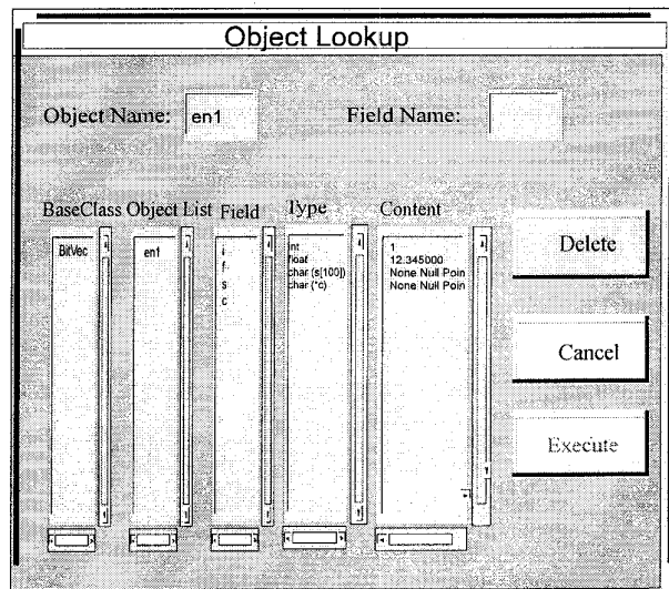
Figure 5. Menu for Object Lookup
