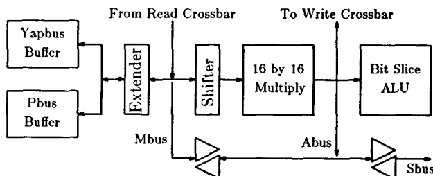
Figure 3: Chap Processing Element
