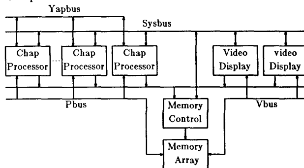
Figure 1: Compositor Communications Channels
