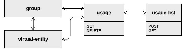
(b) The processes from UC1 are mapped to POST /usage and DELETE /usage/{id} .
