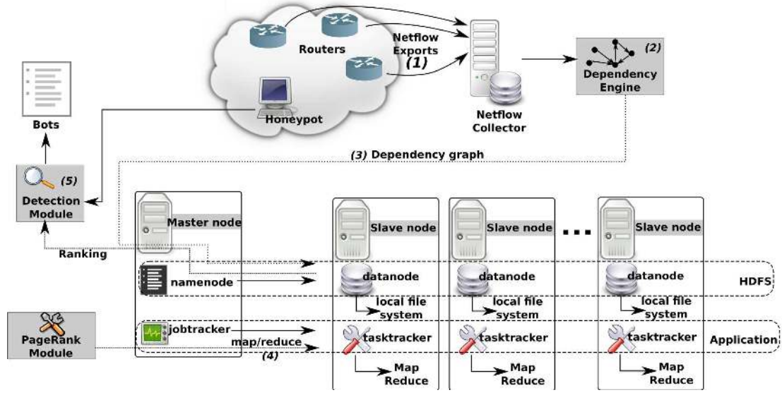
Fig. 1: BotCloud framework
