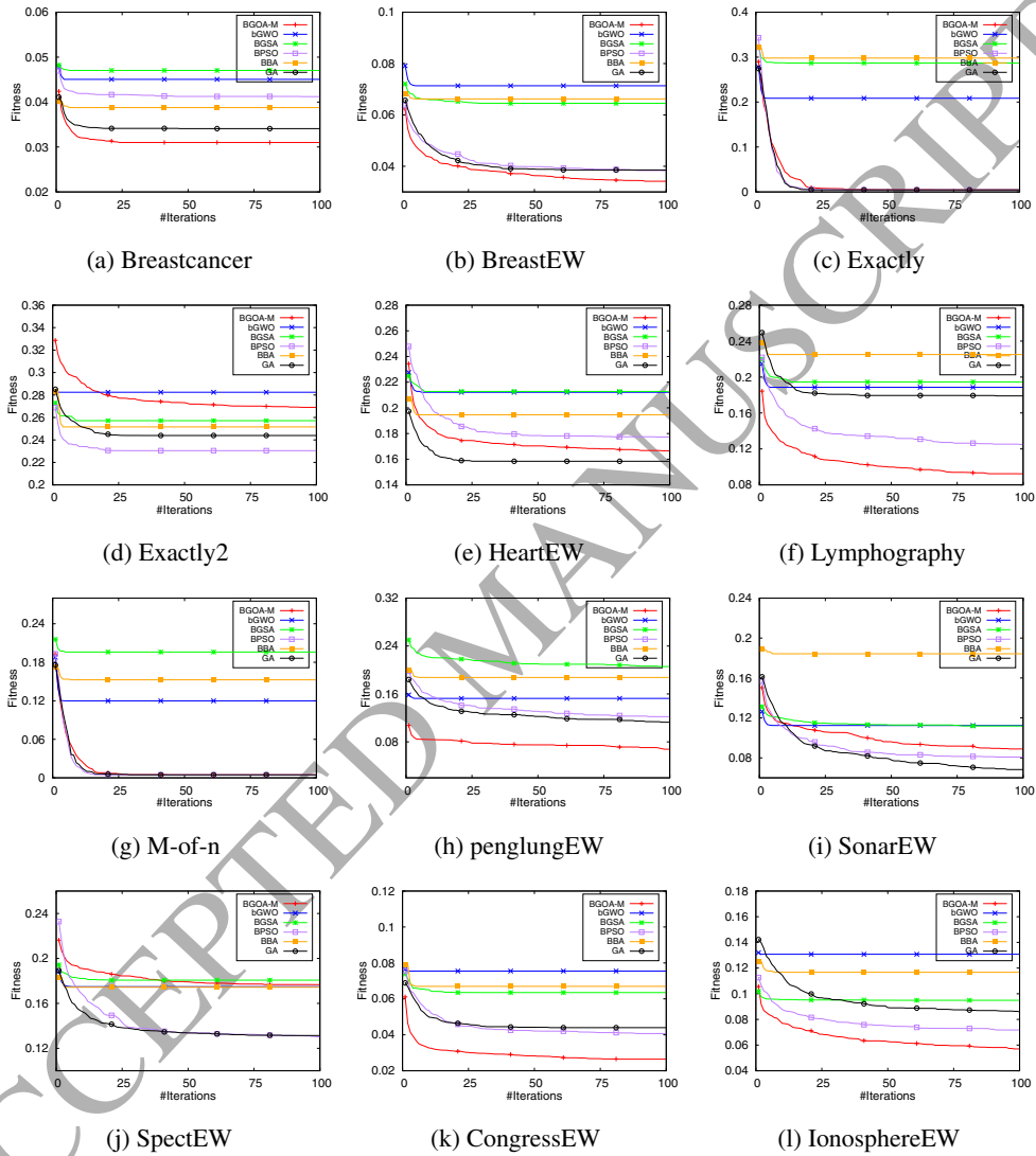
Figure 8: Convergence curves for BGQA-M and other state-of-art methods for Breastcancer, BreastEW, Exactly, Exactly2, HeartEW, Lymphography, M-of-n, penglungEW, SonarEW, SpectEW, CongressEW and IonosphereEW datasets.
