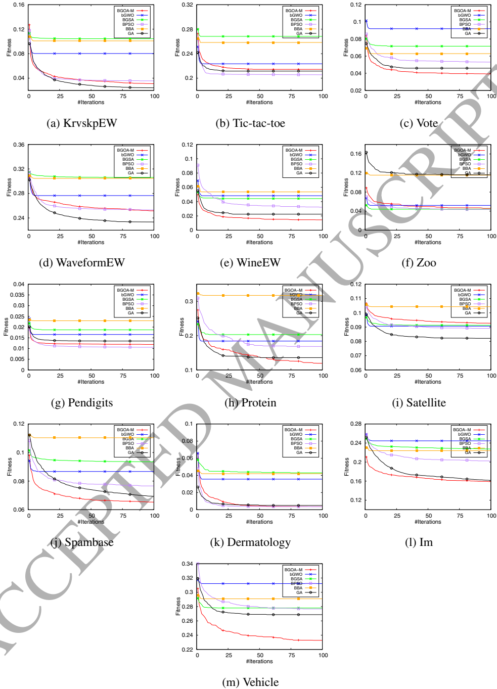
Figure 9: Convergence curves for BGOA-M and other state-of-art methods for KrvskepEW, Tic-tac-toe, Vote, WaveformEW, WineEW, Zoo, Pendigits, Protein, Satellite, Spambase, Dermatology, Im, Vehicle datasets.
