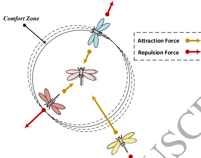
Figure 1: Primitive corrective patterns between individuals in a swarm of grasshoppers.
