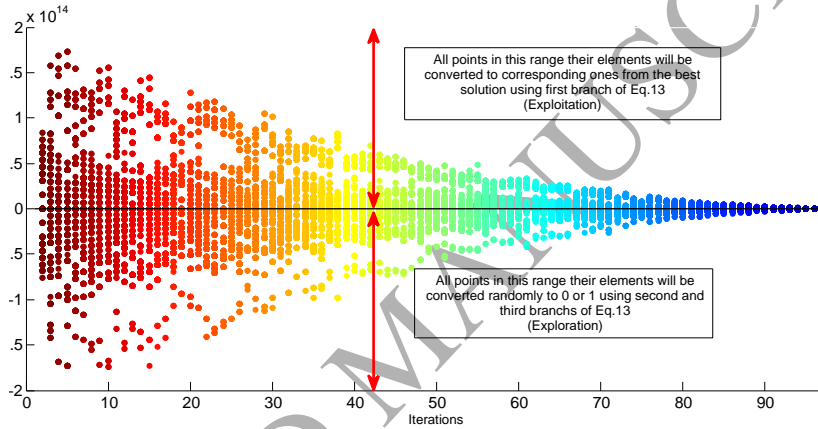
Figure 3: Transfer mechanism in BGOA
