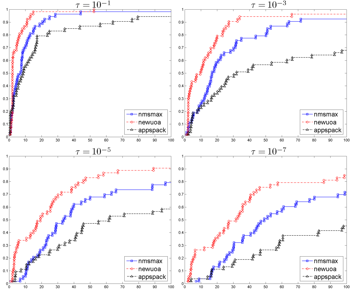
Figure 5.1: Data profiles for the smooth problems \mathcal{P}_S show the percentage of problems solved as a function of a computational budget of (simplex) gradients.
