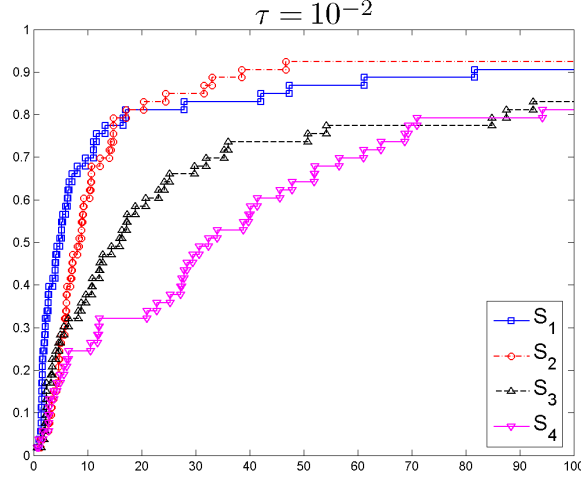
Figure 2.2: Sample data profile for derivative-free solvers.
