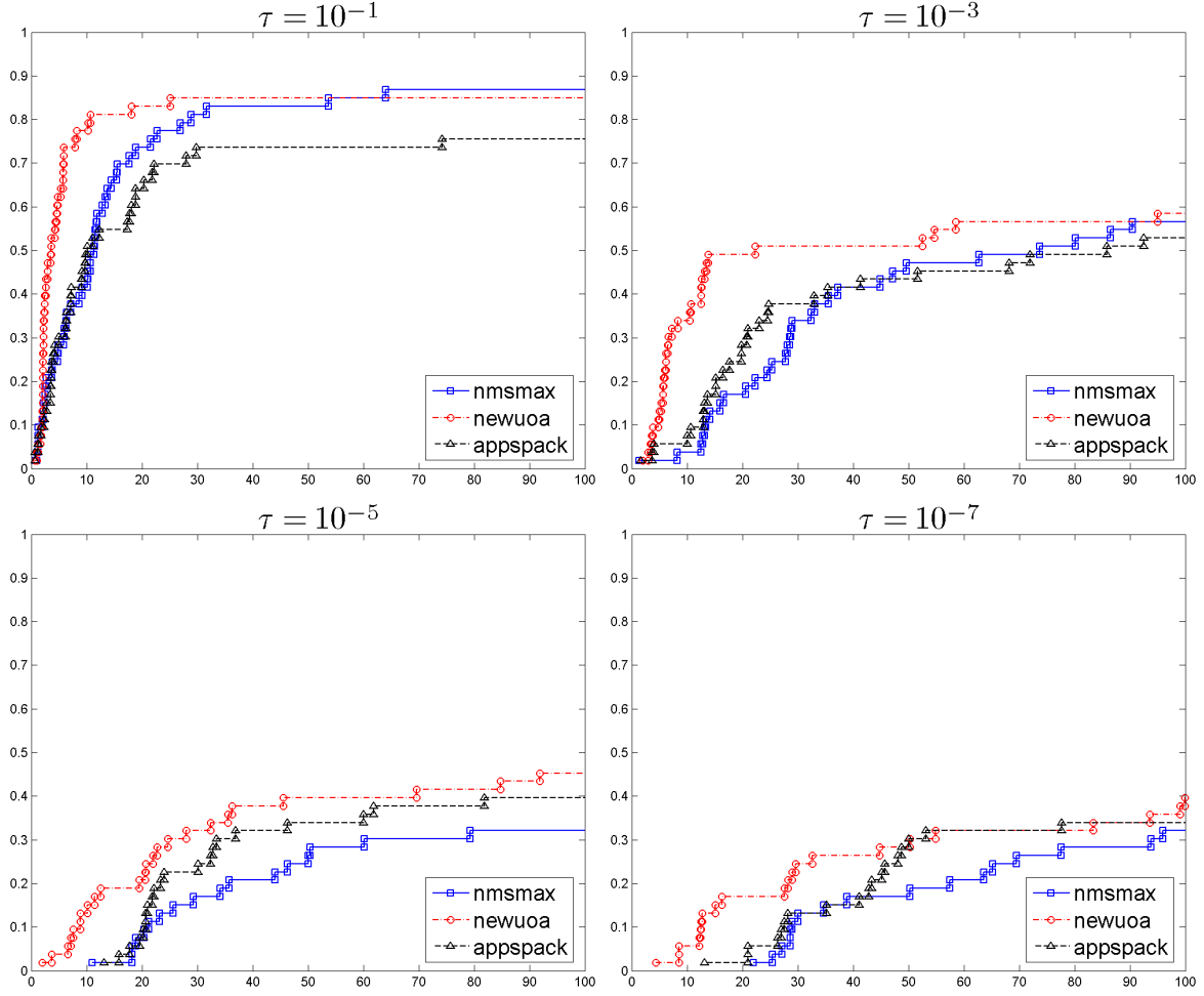
Figure 5.5: Data profiles for the piecewise-smooth problems \mathcal{P}_{PS} show the percentage of problems solved as a function of a computational budget of (simplex) gradients.
