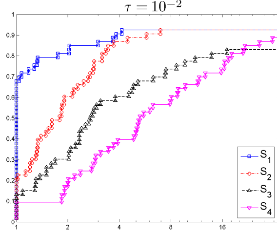
Figure 2.1: Sample performance profile (logarithmic scale) for derivative-free solvers.
