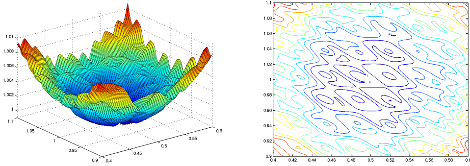
Figure 4.1: Plots of the noisy quadratic (4.5) on the box [0.4, 0.6] \times [0.9, 1.1] . Surface plots (left) and level sets (right) show the oscillatory nature of f .
