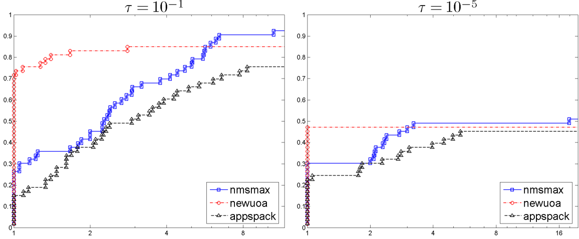
Figure 5.6: Performance profiles (logarithmic scale) for the piecewise-smooth problems \mathcal{P}_{PS} .
