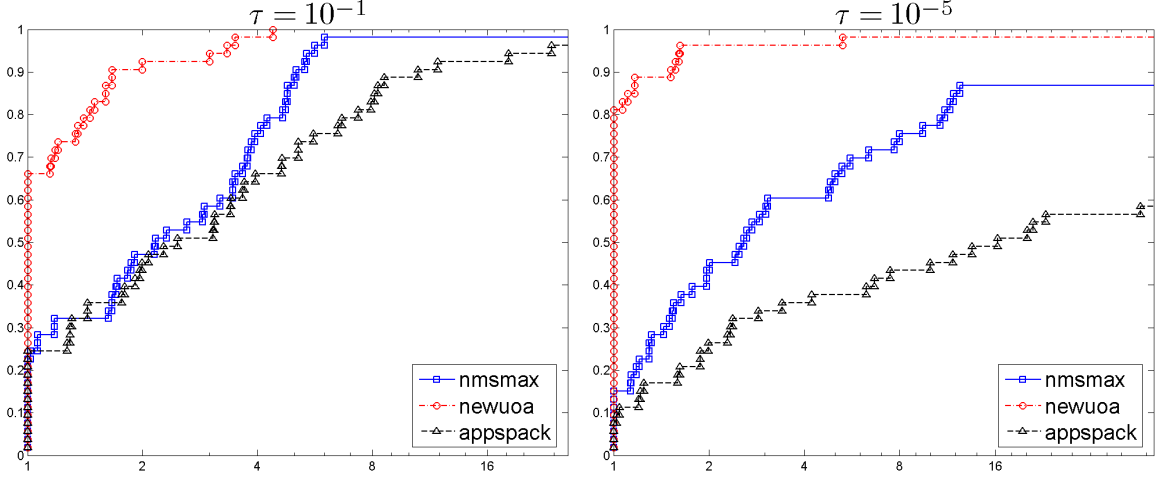
Figure 5.2: Performance profiles (logarithmic scale) for the smooth problems \mathcal{P}_S .
