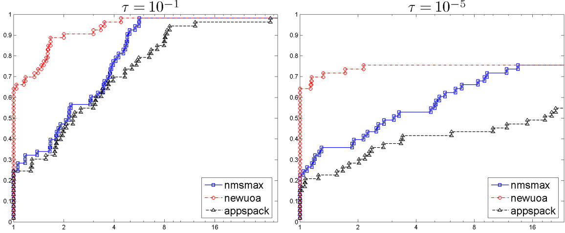
Figure 5.4: Performance profiles (logarithmic scale) for the noisy problems \mathcal{P}_N .
