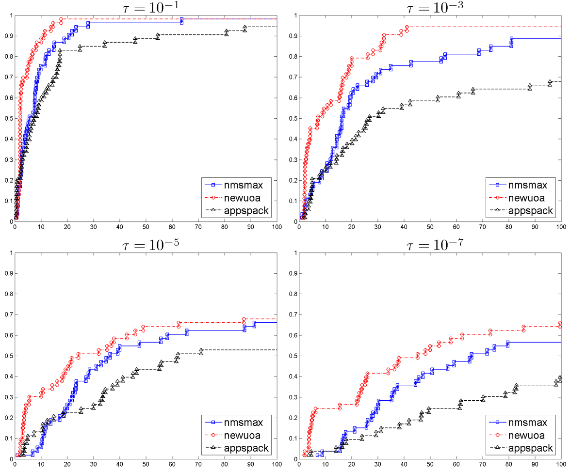
Figure 5.3: Data profiles for the noisy problems \mathcal{P}_N show the percentage of problems solved as a function of a computational budget of (simplex) gradients.
