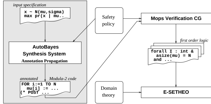
Fig. 1. The AUTOBAYES/CC system architecture
