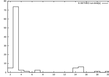
Fig. 2. Left , excerpt of annotated code produced by AUTOBAYES/CC. Annotations are enclosed in (*{...}*) . Right , distribution of E-SETHEO proof times (% solved over runtime in seconds).
