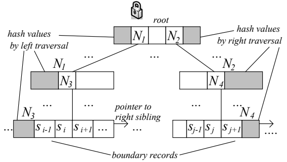
Figure 2 Example of Merkle B-tree
