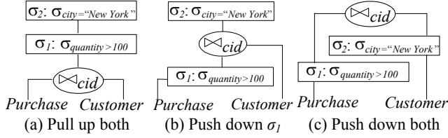
Figure 16 Three query plans for Q_4
