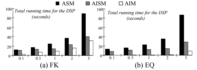
Figure 22 Query cost for the DSP vs. |S|/|R|
