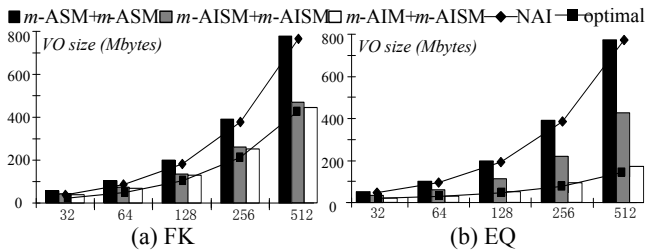
Figure 23 VO size vs. tuple size
