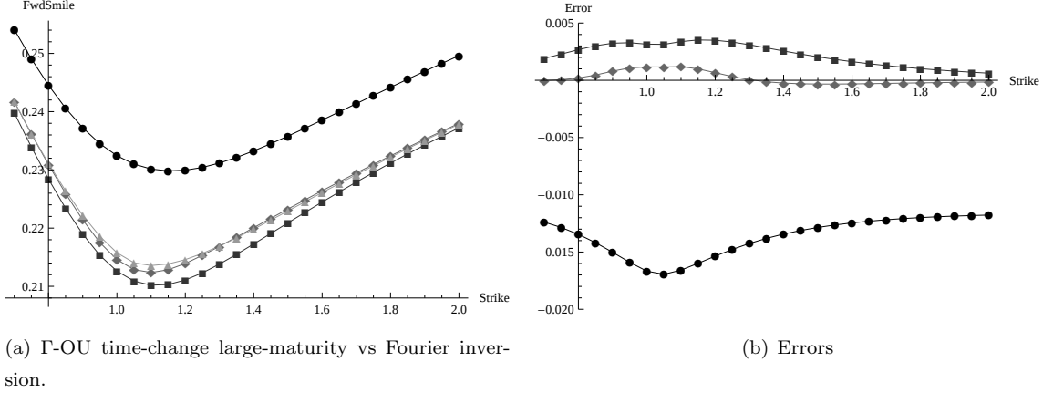
FIGURE 7. In (a) circles, squares and diamonds represent the zeroth, first and second order asymptotics respectively in proposition 3.19 and triangles represent the true forward smile using Fourier inversion for a variance gamma model time-changed by a \Gamma -OU process. In (b) we plot the differences between the true forward smile and the asymptotic. We use t = 1 and \tau = 3 with the parameters C = 6.5 , G = 11.1 , M = 33.4 , v = 1 , \alpha = 0.6 , d = 0.6 , \lambda = 1.8 .
