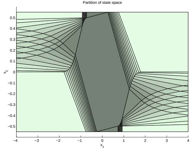
Figure 4: Exact polyhedral partition of the state space, N = 10 .
