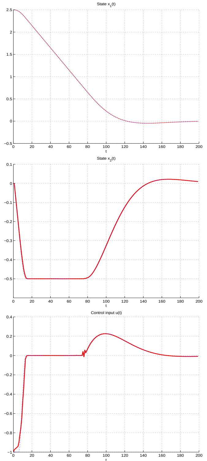
Figure 5: Simulation where the dashed curves are with the exact controller, and the solid curves are with the approximate controller, with N = 10 and \sqrt{\epsilon_r} = 0.5 .
