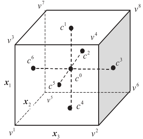
Figure 2: Illustration of the heuristic splitting rule
