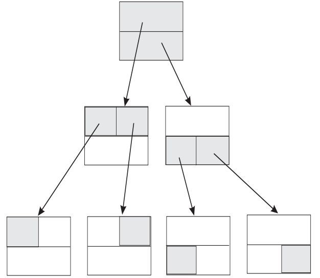
Figure 1: k-d -tree partition of a rectangular region in \mathbb{R}^2 .
