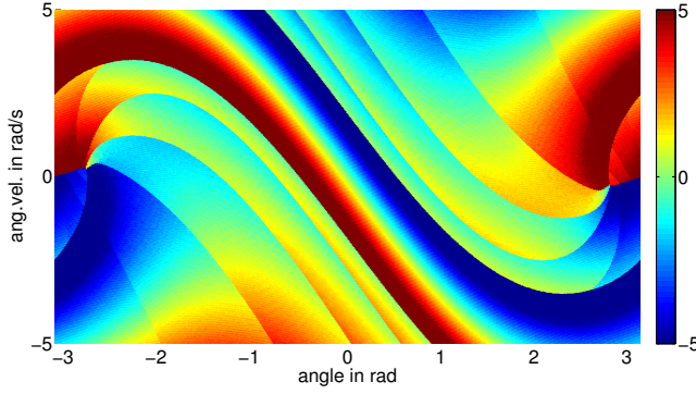
Fig. 2. Optimal policy for a discretized system with 6.2 \times 10^5 states and 125 controls. Discontinuities at the boundary of the central band are caused by the dynamics. Due to temporal discretization, stripes of optimal controls with discontinuous borders appear in the upper right and lower left corners. Red and blue colors show positive and negative controls, respectively.
