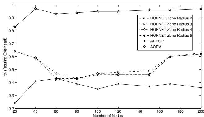
Fig. 9. Routing Overhead
