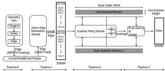
Figure 4. Architecture of Implemented 2D Vector Graphics Engine
