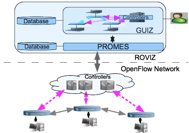
Figure 1: ROVIZ: Network Visualization Framework
