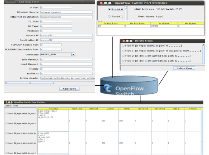
Figure 2: GUIZ: Interactive Visual Menu
