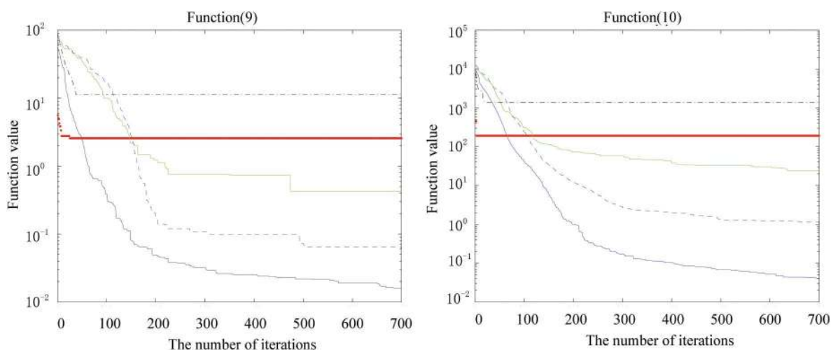
Fig 6. The fitness value of various algorithms for Alpine and Powell during increasing iterative times.
