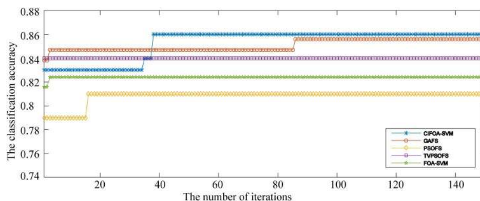
Fig 16. The convergence curves generated for fold #5 run by the five methods for German Credit Data (GCD).
