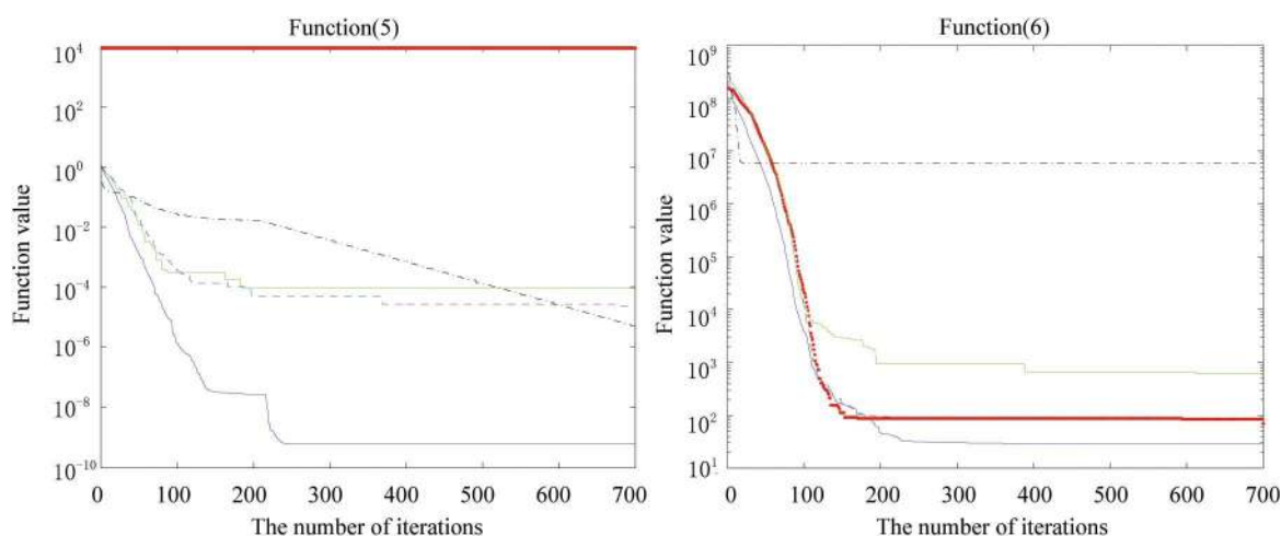
Fig 4. The fitness value of various algorithms for Rosenbrock and Sum of different power during increasing iterative times.
