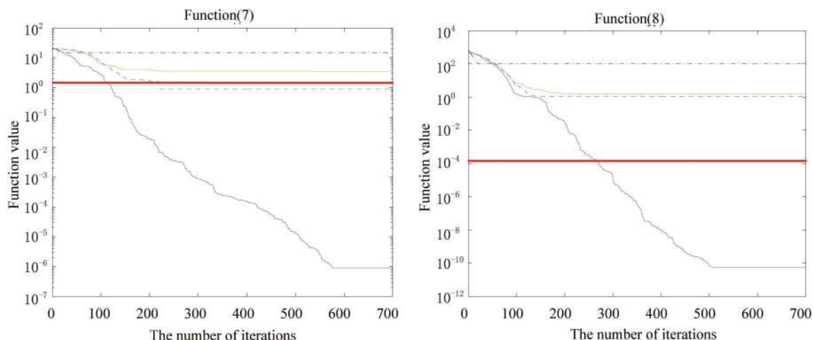
Fig 5. The fitness value of various algorithms for Ackley and Griewank during increasing iterative times.
