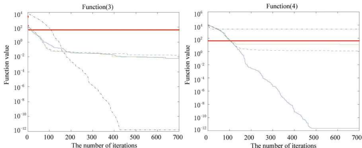
Fig 3. The fitness value of various algorithms for Quartic and Sum squares during increasing iterative times.
