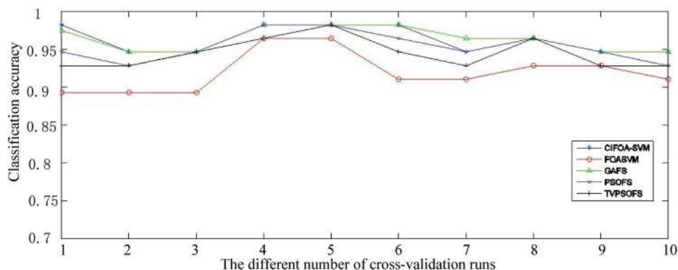
Fig 9. The classification accuracy achieved for each fold run by various methods for the WDBC-1995.
