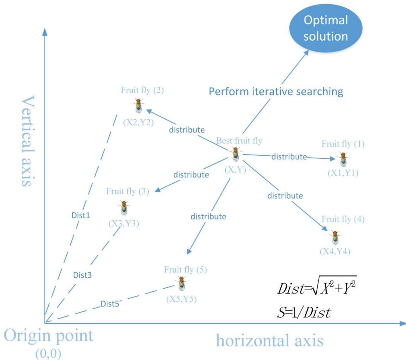
Fig 1. The food searching process of a fruit fly swarm.
