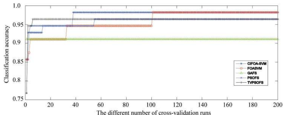
Fig 12. The convergence curves generated for the fold #3 run by the five methods for the WDBC-1995.
