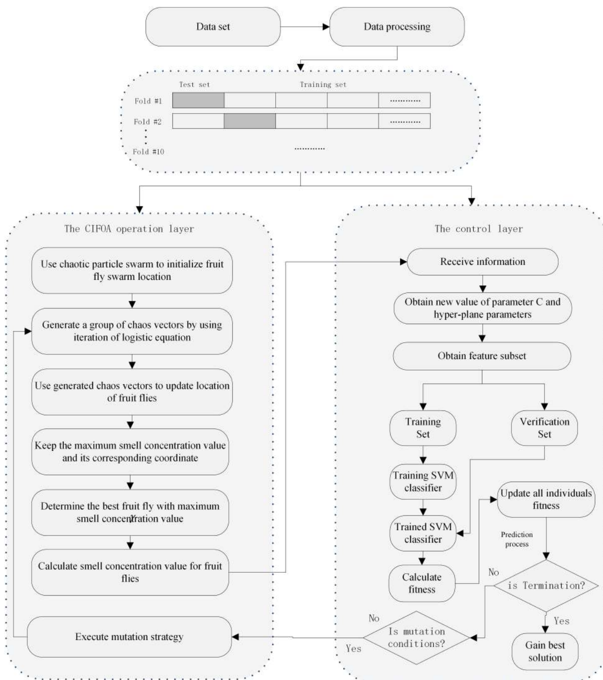
Fig 8. The basic process of the proposed framework.
