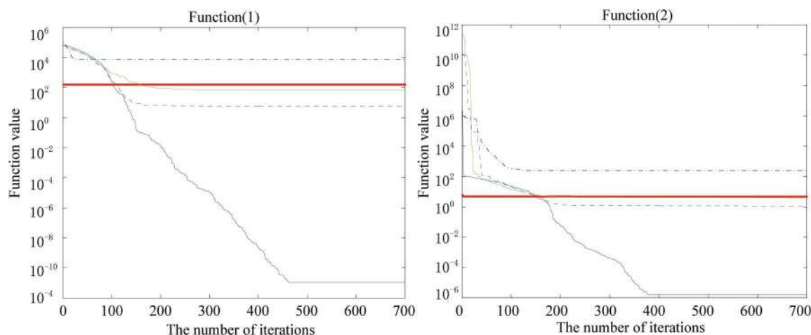
Fig 2. The fitness value of various algorithms for Sphere and Schwefel's problem 2.22 during increasing iterative times.
