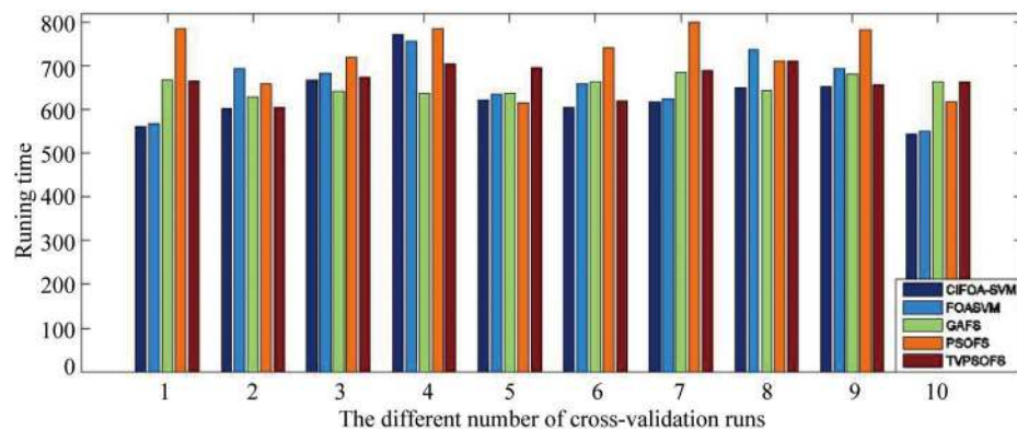
Fig 15. The required running time in seconds for each run by the five methods for German Credit Data (GCD).
