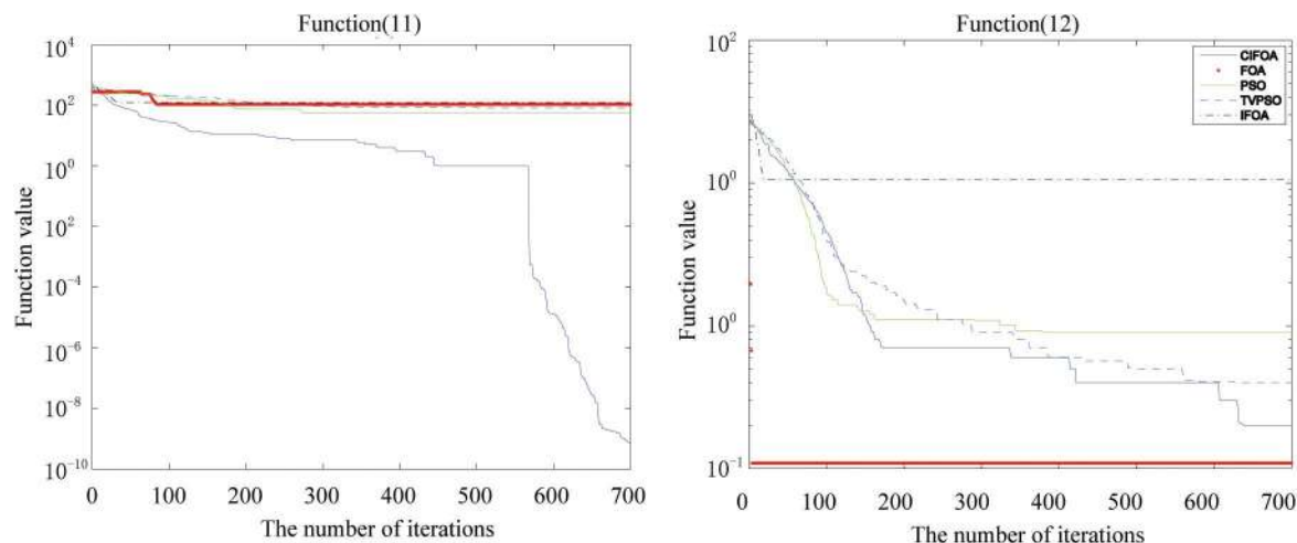
Fig 7. The fitness value of various algorithms for Rastrigin and the Solomon problem during increasing iterative times.
