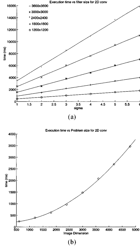
Figure 8. (a) The plot of execution time vs filter size. (b) Execution time for various image size.
