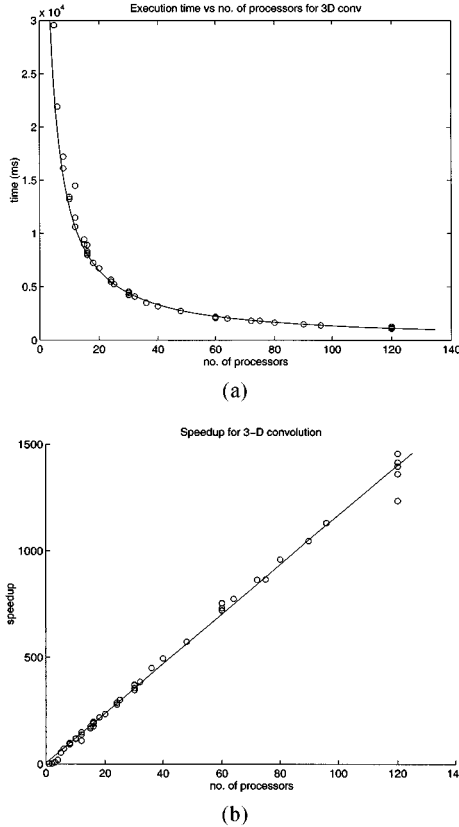
Figure 9. Impact of no. of processors on the execution time.
