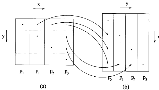
Figure 1. Redistribution of the image.
