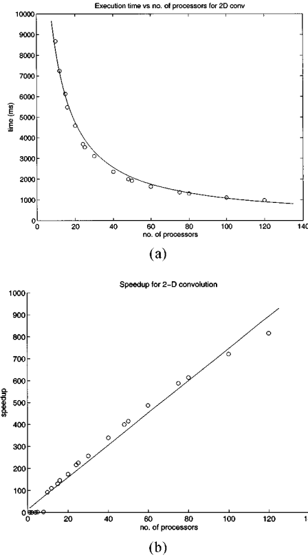
Figure 7. Impact of no. of processors on the execution time.
