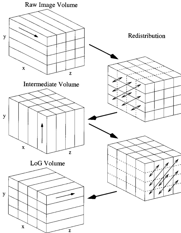
Figure 4. Redistribution of image volume.
