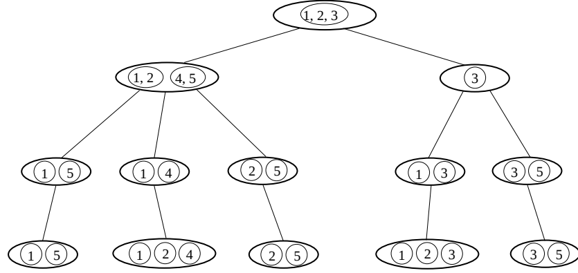
Figure 1: Transversal tree of the hypergraph \mathcal{H} = \{\{1, 2, 3\}, \{3, 4, 5\}, \{1, 5\}, \{2, 5\}\} . The tree is visited in preorder.
