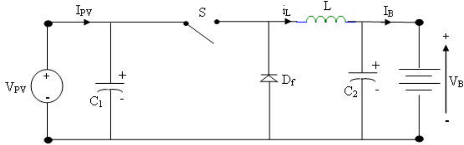
Fig. 3: The step-down DC-DC converter
