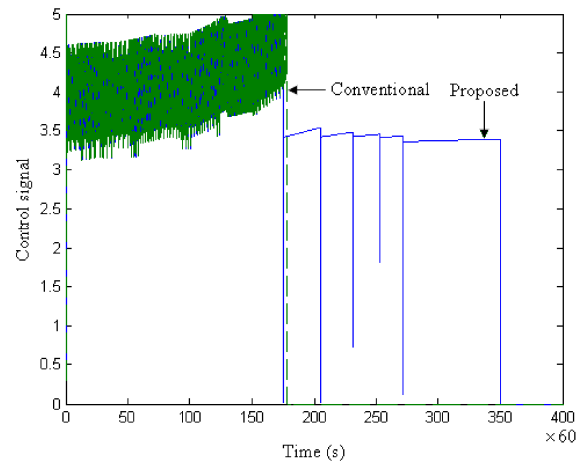
Fig. 7: Control signal during the charging time
