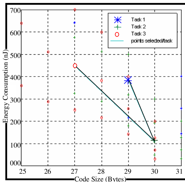
Figure 6. Code Size Vs Energy Consumption (Matlab simulation)
