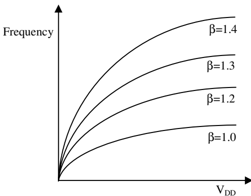
Figure 3. Variation of V_{DD} and frequency F
