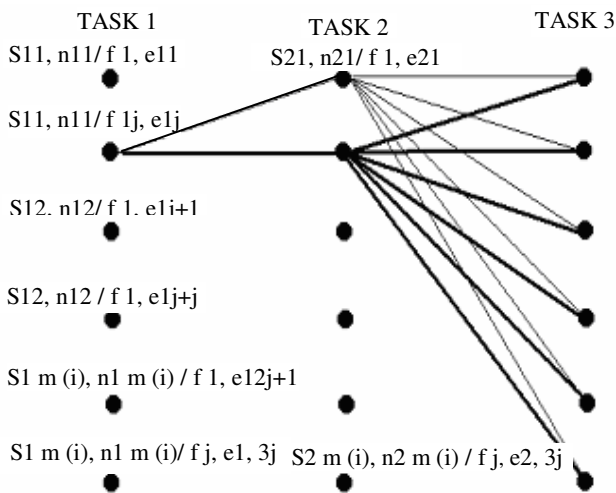
Figure 5. Schematic procedure to obtain combinations of triple trade off tuples
