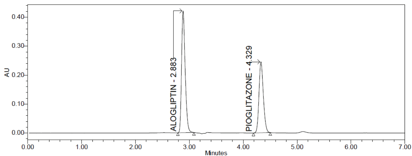
Figure 2. Typical HPLC chromatogram of alogliptin and pioglitazone
