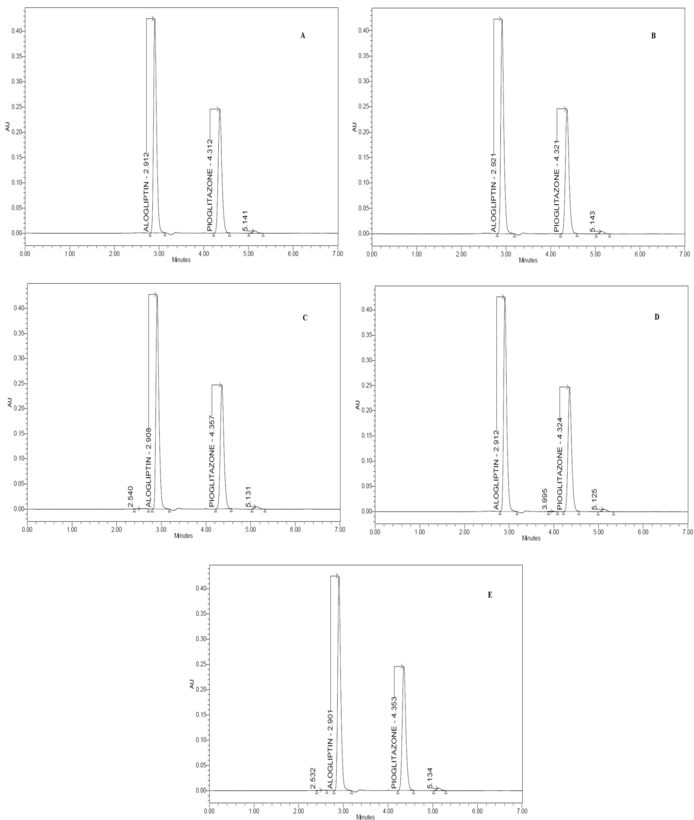
Figure 4. Chromatogram of tablet sample (A) Treated with 0.1 N HCl (B) Treated with 0.1 N NaOH (C) Treated with 30% H 2 O 2 (D) Exposed to 105°C (E) Exposed to sunlight
