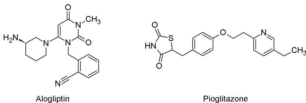
Figure 1. Chemical structures of alogliptin and pioglitazone
